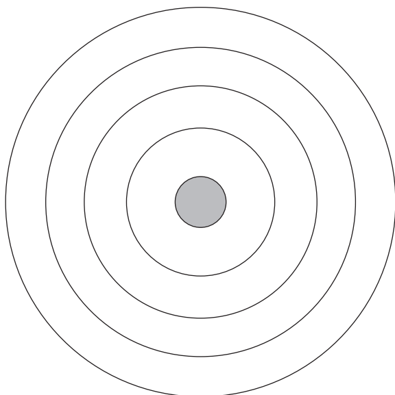
atom of calcium
