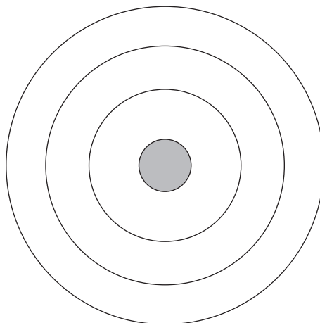
atom of chlorine
